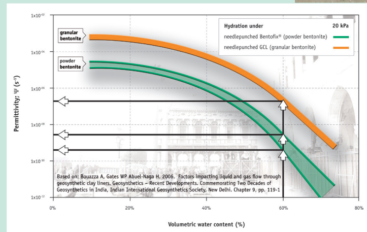
Figure 2 Performance of powdered Bentofix® bentonite compared to granular bentonite in correlation to water content and gas permeability
