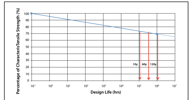
Fig. 2 Creep Rupture Curve for ACEGrid® Geogrid
