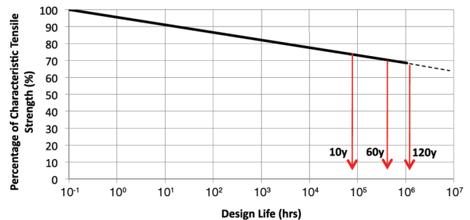
Fig. 2 Creep Rupture Curve for ACETex® PET Woven Geotextile
