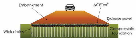
B. Use wick drains to accelerate settlement
