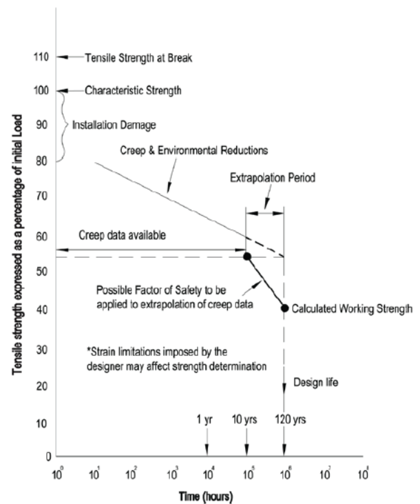
Fig. 1 Partial Factor Reductions to be Considered in Long Term Strength Derivation
