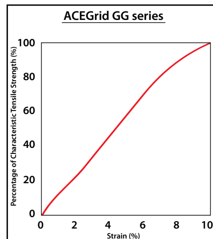
Fig. 3 short term tensile strength-strain relationship for ACEGrid® Geogrid.
