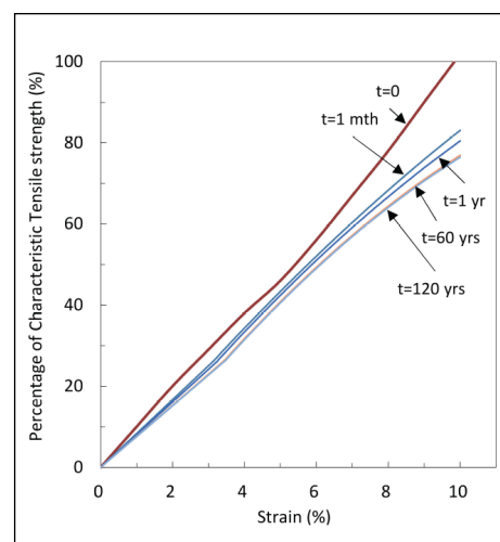
Fig. 4 long term tensile strength-strain-time relationship for ACEGrid® Geogrid isochronous curves.
