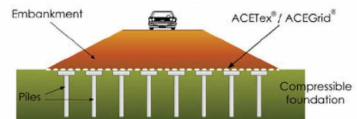
C. Use foundation treatment (piling) to prevent settlement
