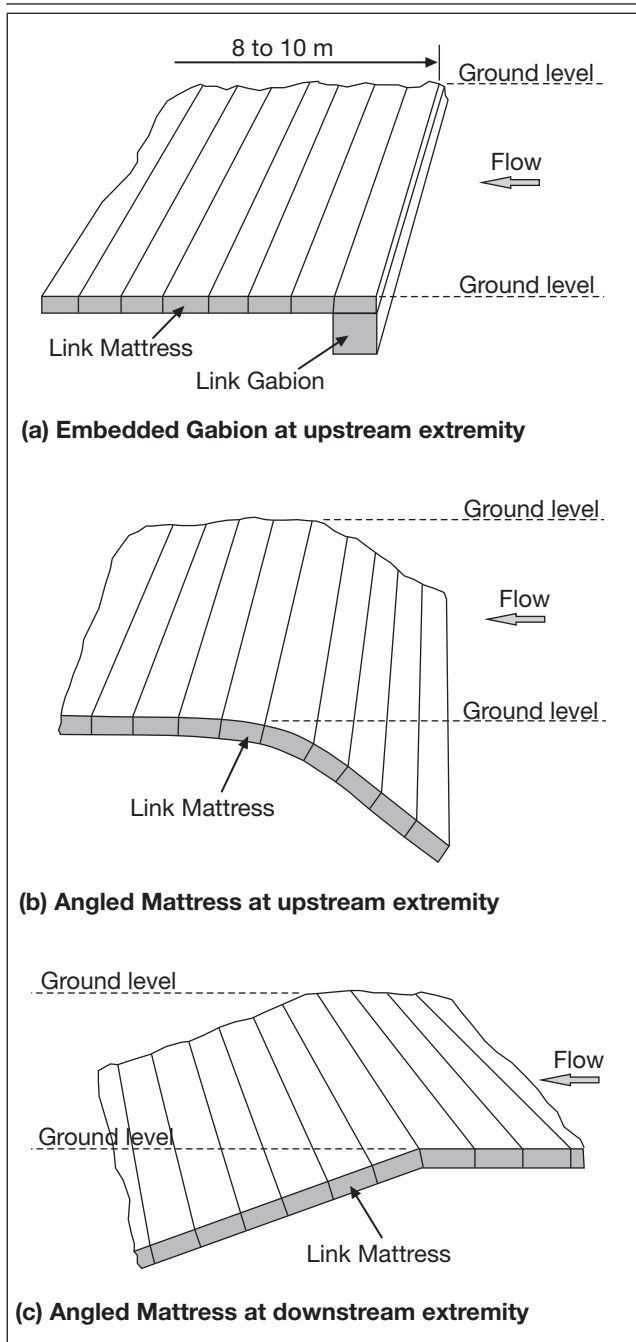
Figure 28 - Extremity details for stream bed protection.
