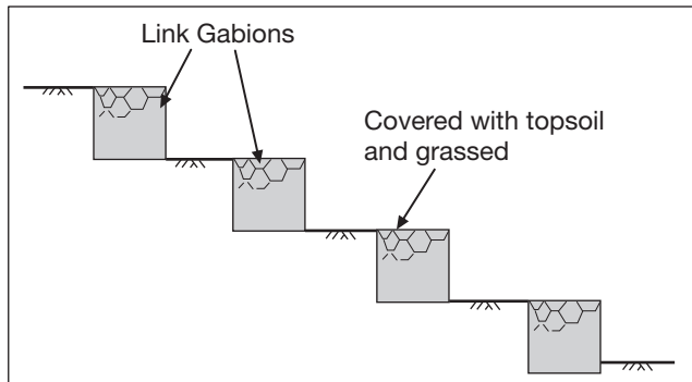
Figure 18 - using Link Gabions for landscaping slopes.
