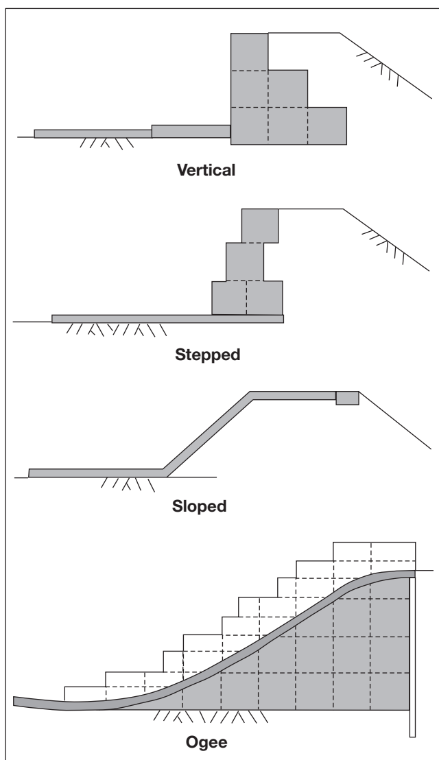
Figure 32 - Weir types using Link Gabions and Mattresses.
