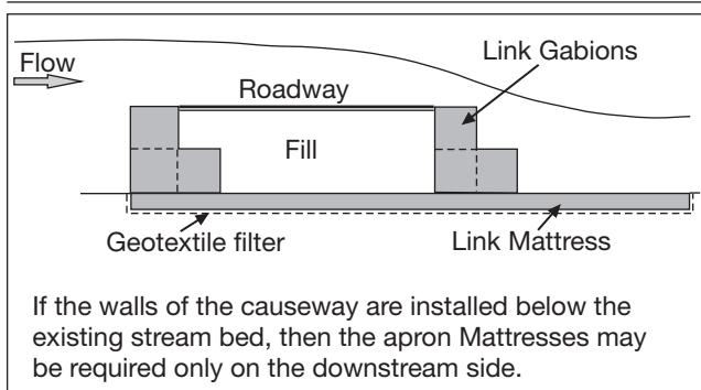
Figure 35 - Low cost design using Link Gabions for low level crossings.
