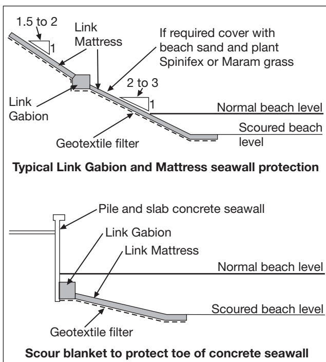
Figure 38 - Typical layouts of Link Gabions and Mattresses for beach protection seawall works.
