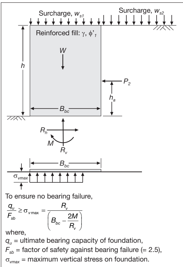
Figure 13 - Stability against bearing failure.
