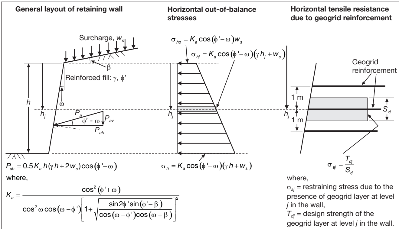
Figure 14 - Determination of required geogrid reinforcement design strengths in a Link Gabion faced reinforced soil wall.
