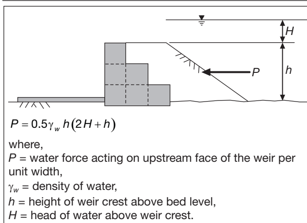
Figure 33 - Horizontal water force acting on upstream face of weirs.
