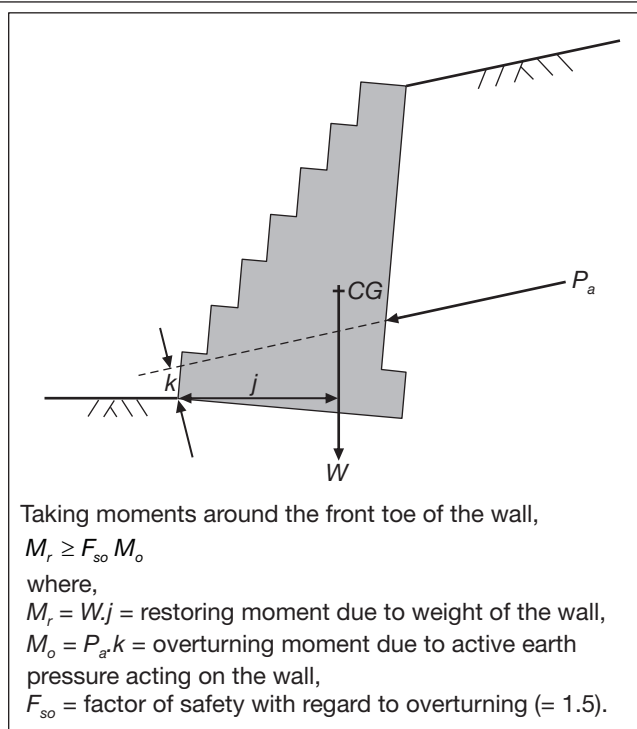
Figure 6 - Stability against overturning.
