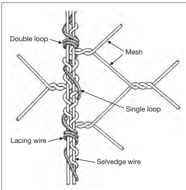
Figure 40 - Link Gabion and Mattress lacing technique.
