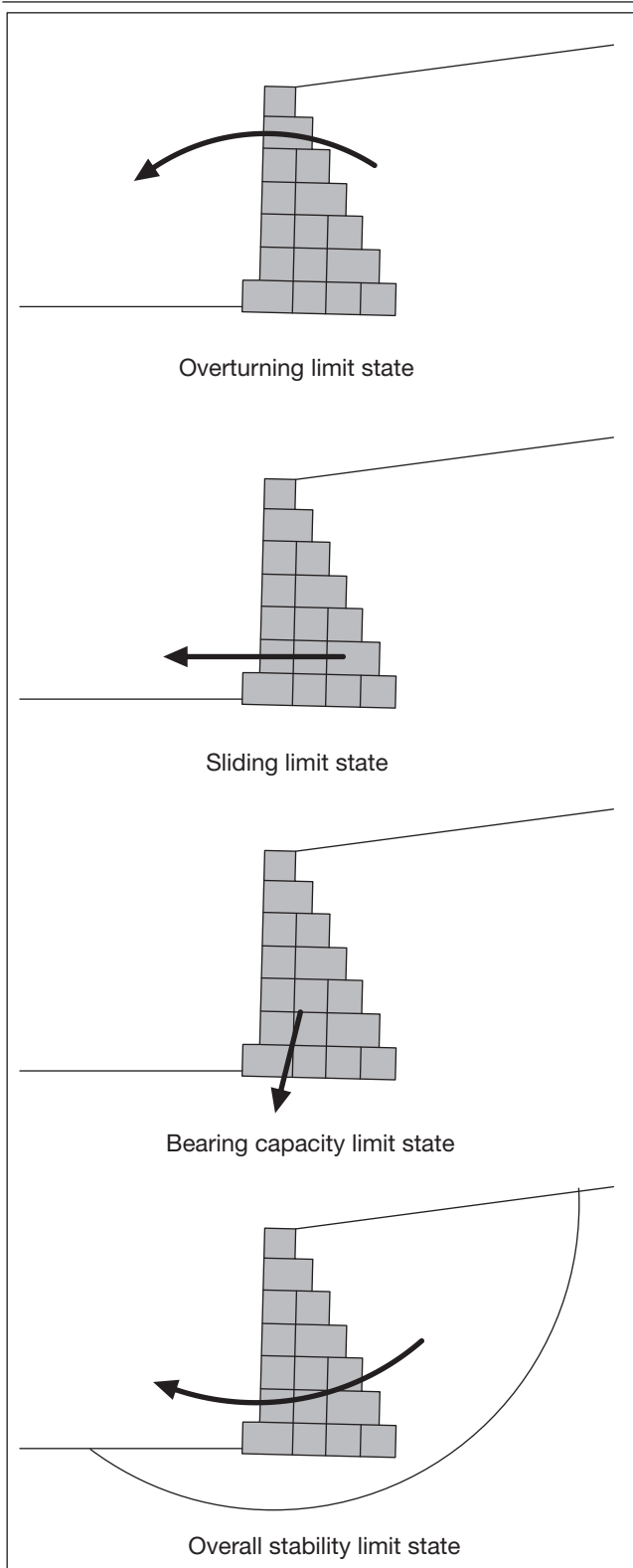
Figure 5 - Design limit states for Link Gabion gravity retaining walls.
