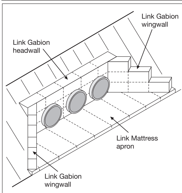
Figure 29 - Typical use of Link Gabions and Mattresses at culvert exits.
