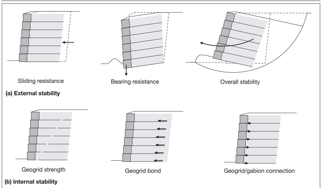
Figure 11 - Design limit states for Link Gabion faced reinforced soil walls.
