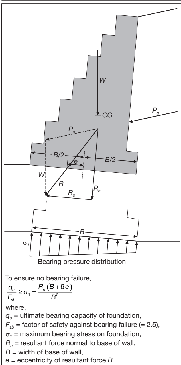
Figure 9 - Stability against bearing failure.
