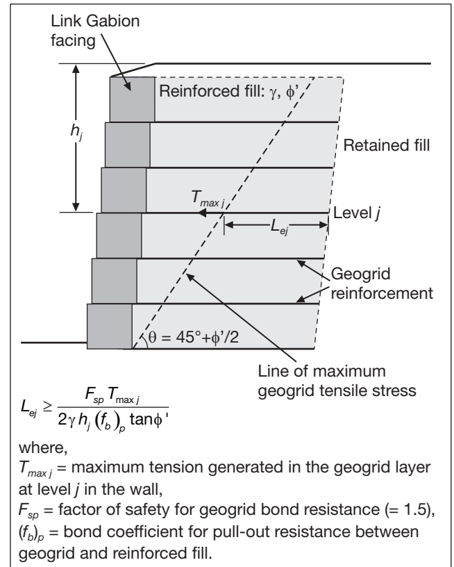
Figure 15 - Required geogrid reinforcement bond length.
