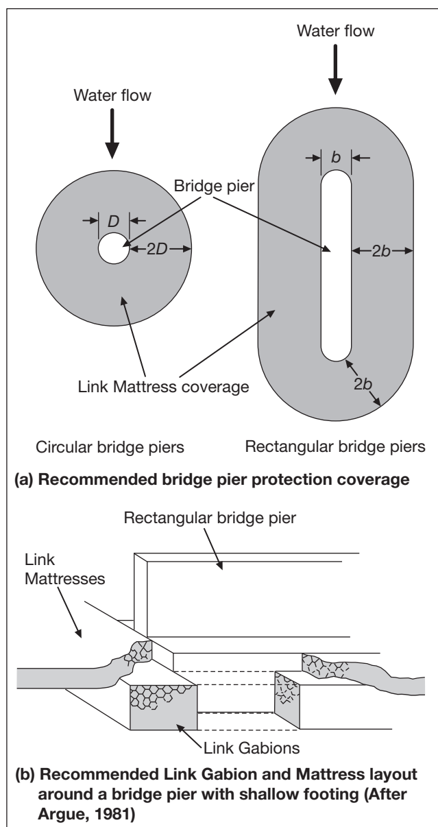
Figure 27 - Link Mattress and Gabion protection around bridge piers.
