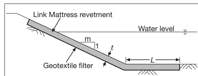
Figure 19 - Link Mattresses used for revetment protection.
