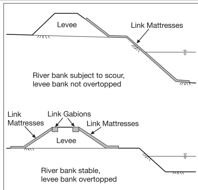
Figure 23 - Use of Link Mattresses to protect levees.
