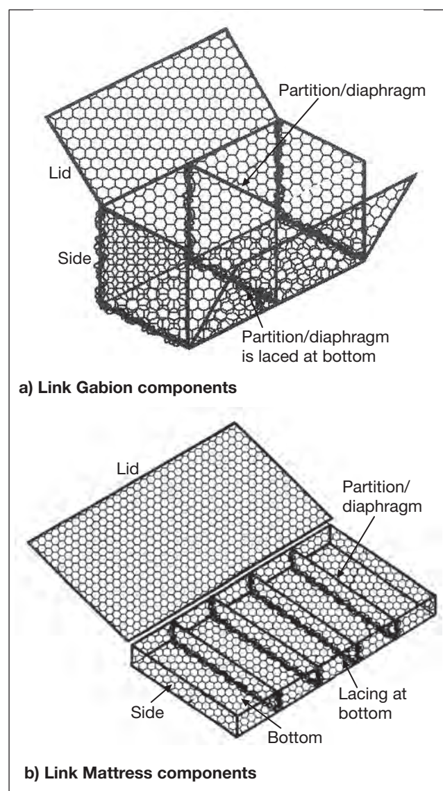
Figure 39 - Link Gabion and Mattress components.
