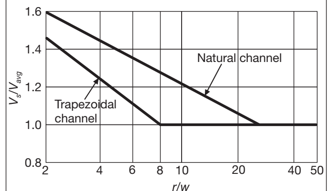
Figure 20 - Determination of Link Mattress thickness requirements for water flows in rivers, channels and streams (After Maynard, 1995).
