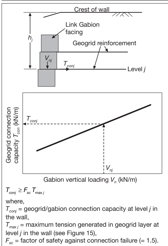
Figure 16 - Geogrid connection capacity determination with Link Gabion facing.
