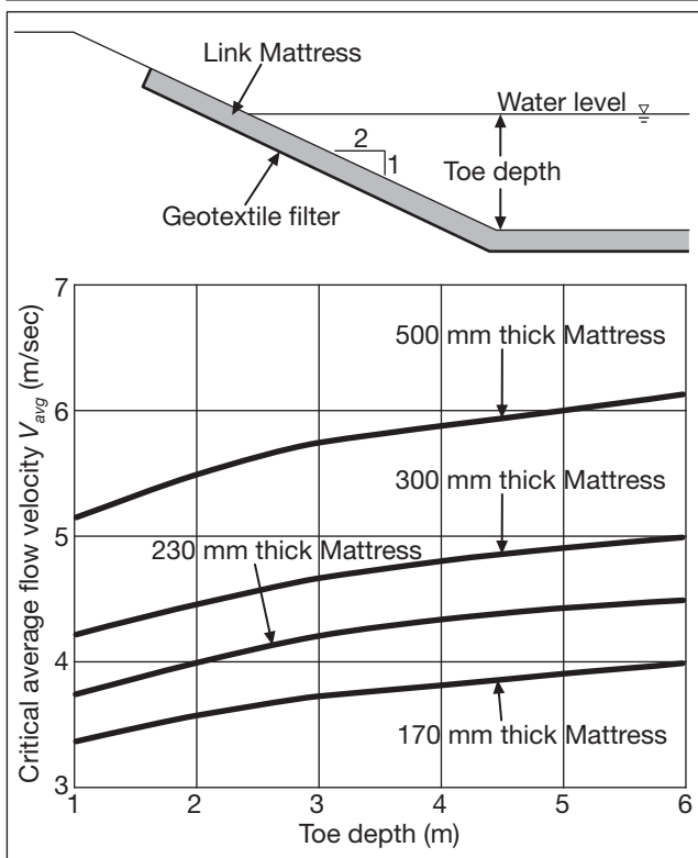
Figure 21 - Critical average flow velocities for different thickness Link Mattresses laid at slope 1V:2H in a straight, natural channel where Froude number \leq 1.5 .
