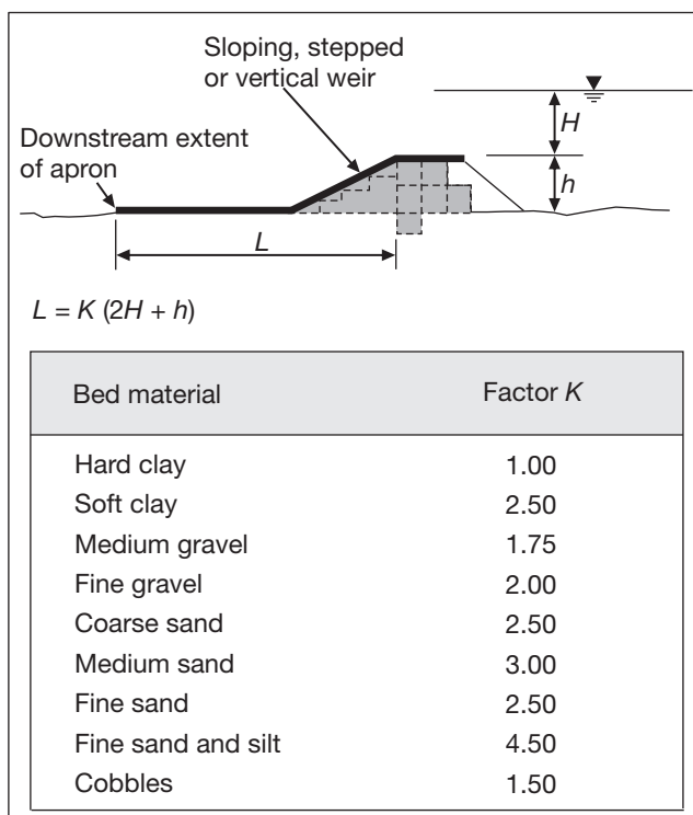
Figure 34 - Link Mattress extent requirements downstream of weirs.
