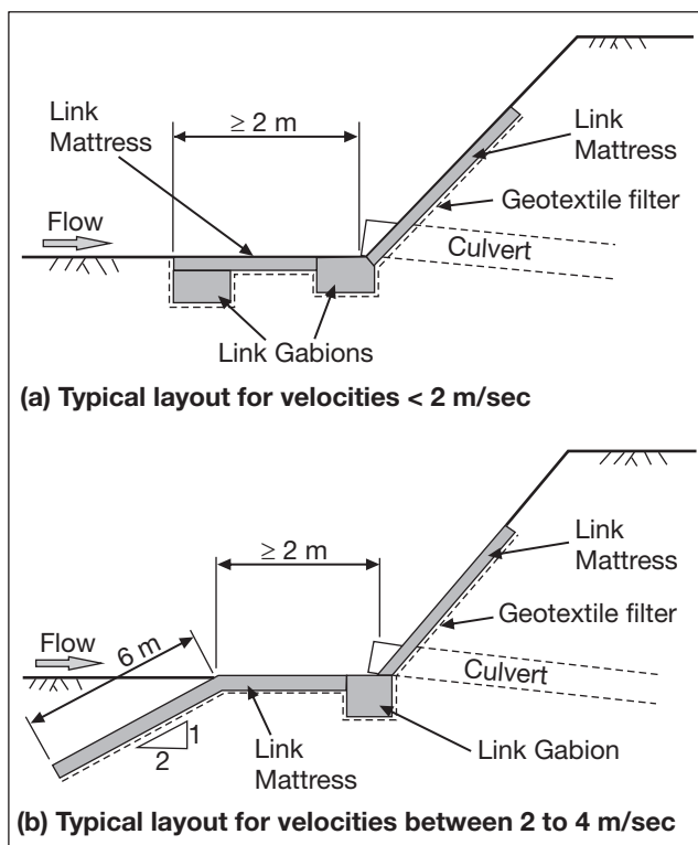
Figure 30 - Link Mattress apron details for local scour protection at entrance to culverts.
