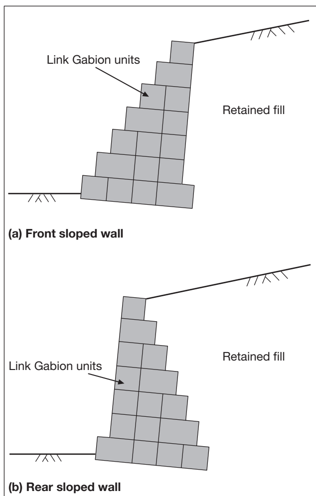
Figure 4 - Two types of Link Gabion gravity walls.
