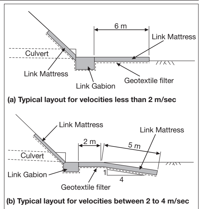
Figure 31 - Link Mattress apron details for local scour protection at culvert outlets.
