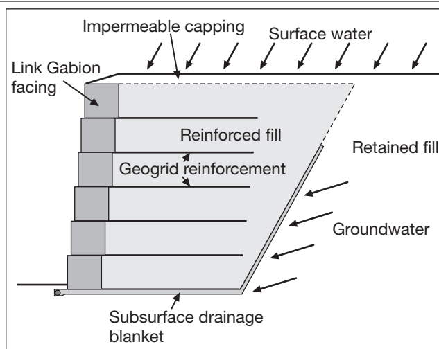
Figure 17 - Protection of reinforced soil wall from surface water and groundwater flows.
