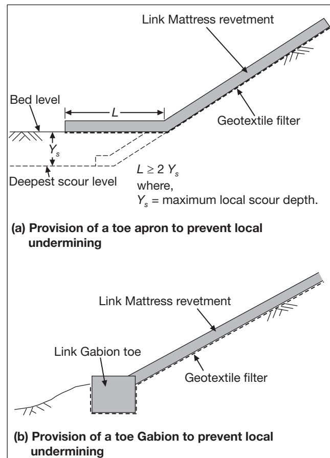
Figure 26 - Toe detailing for abutment protection using Link Mattresses.
