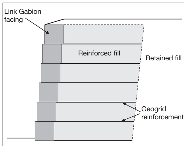
Figure 10 - Typical layout showing the components of a Link Gabion reinforced soil wall.
