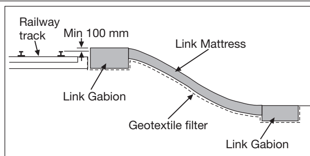
Figure 36 - Detail showing railway embankment protection on downstream face when designed for overtopping by medium to high flows.
