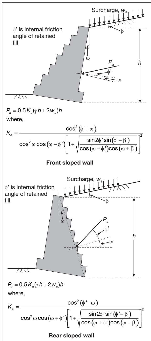
Figure 7 - Calculation of coefficient of active thrust on rear of Link Gabion gravity walls.
