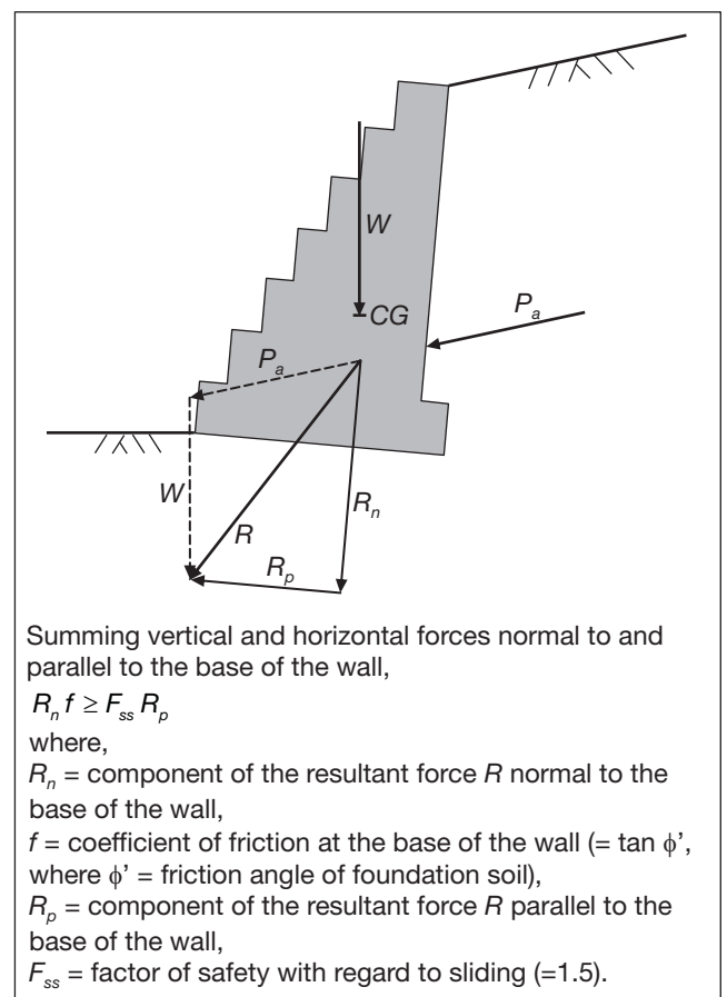
Figure 8 - Stability against sliding.
