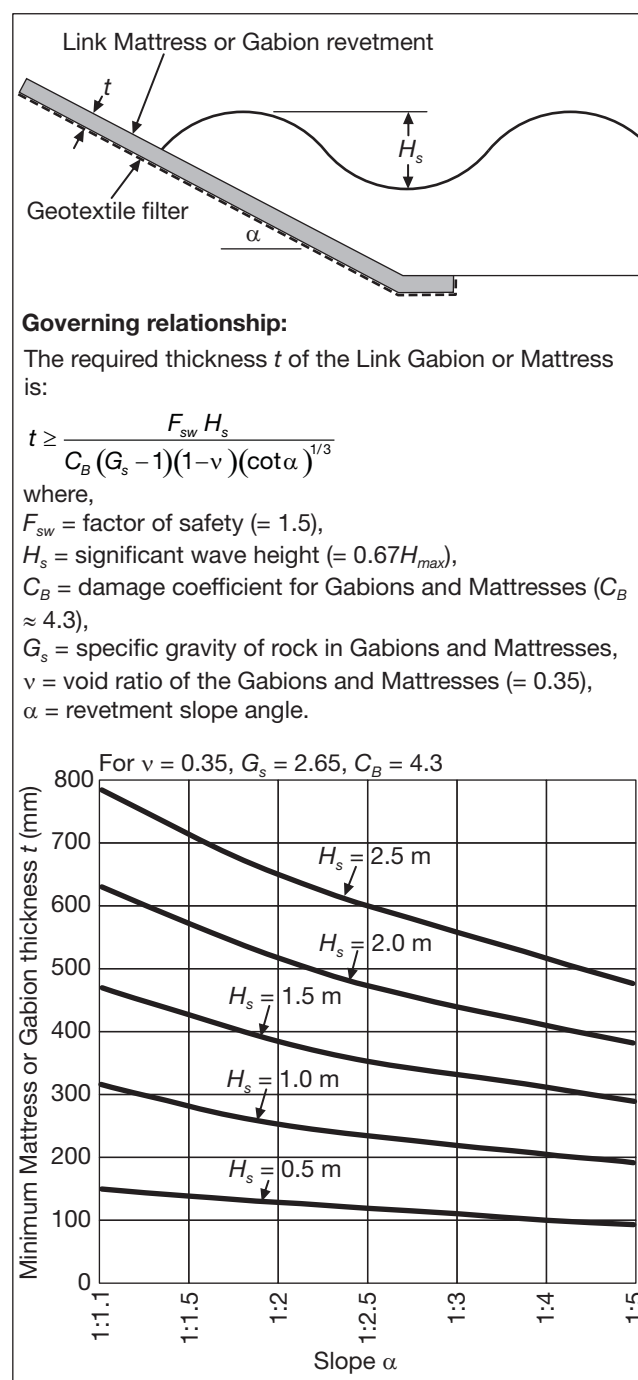
Figure 37 - Link Gabion and Mattress thickness requirements for revetment stability due to waves (After Brown, 1978).
