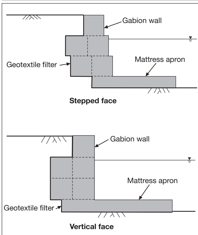
Figure 25 - Typical river and stream training walls.
