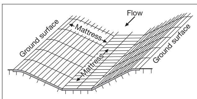
Figure 22 - Arrangement of Link mattresses in rivers, channels and streams.
