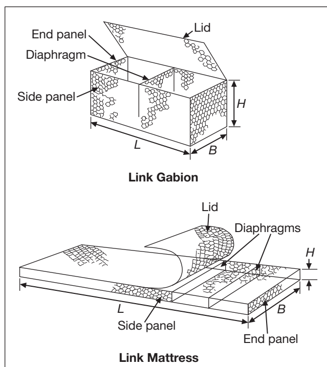
Figure 1- Link Gabions and Mattresses.
