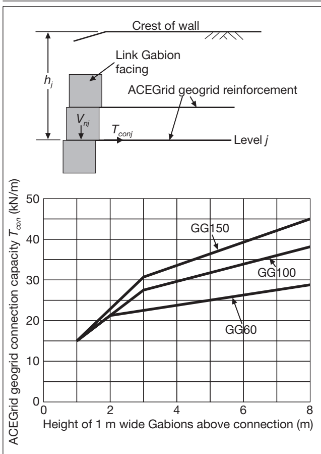
Figure 3 - ACEGrid geogrid connection capacity with 1 m wide Link Gabions.
