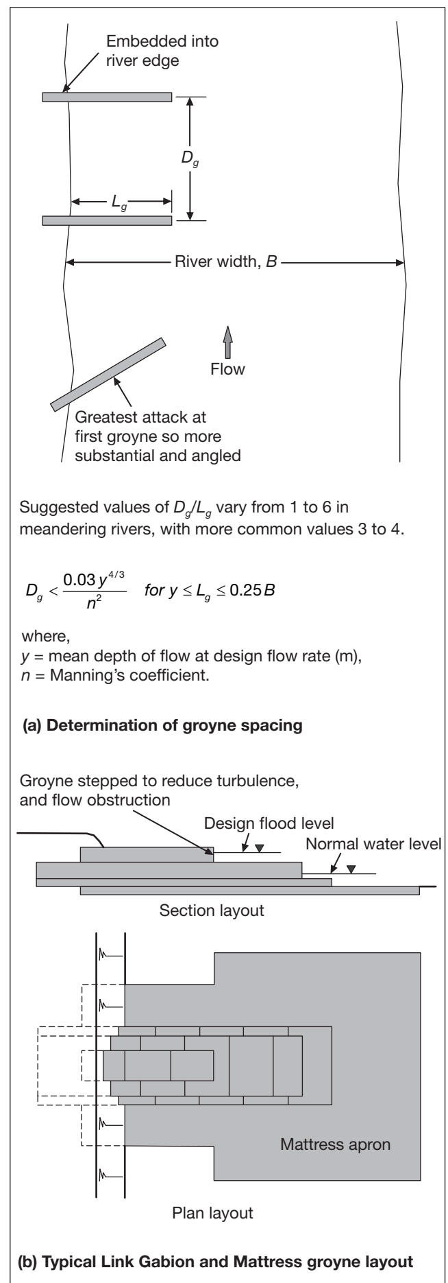
Figure 24 - Dimensions of river groynes using Link Gabions and Mattresses (derived from CIRIA, 2007).
