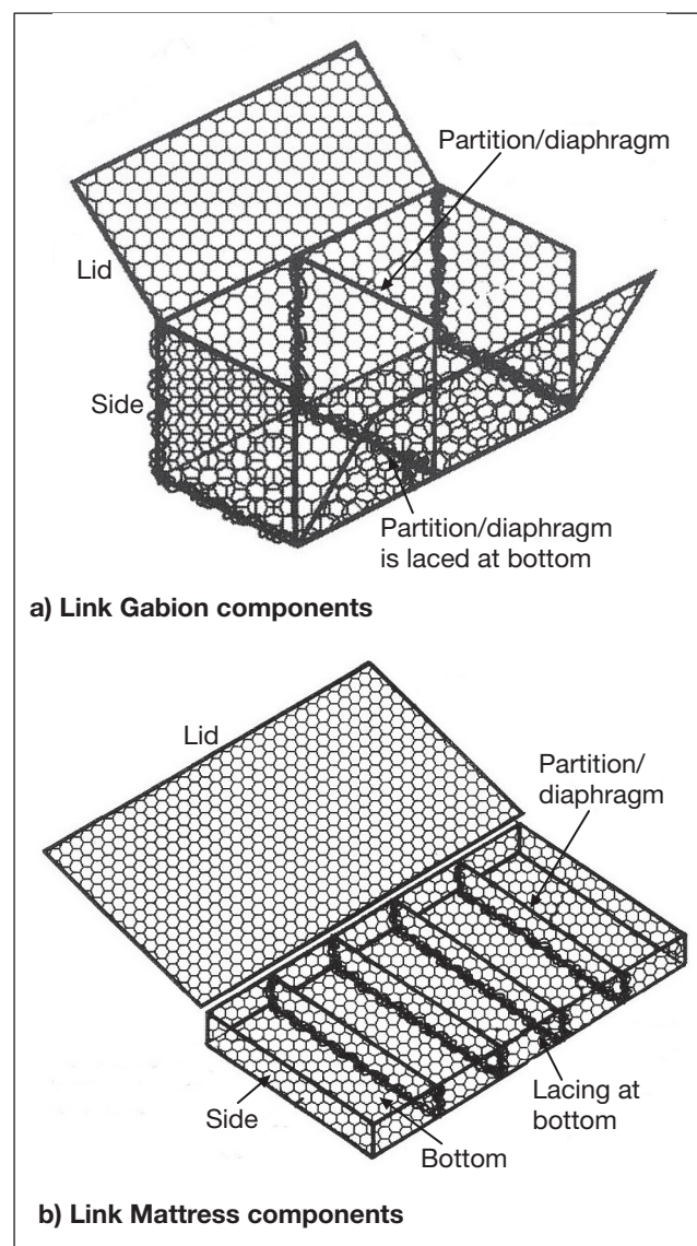
Figure 39 - Link Gabion and Mattress components.
