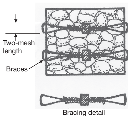
b) Gabion filling and bracing placement
