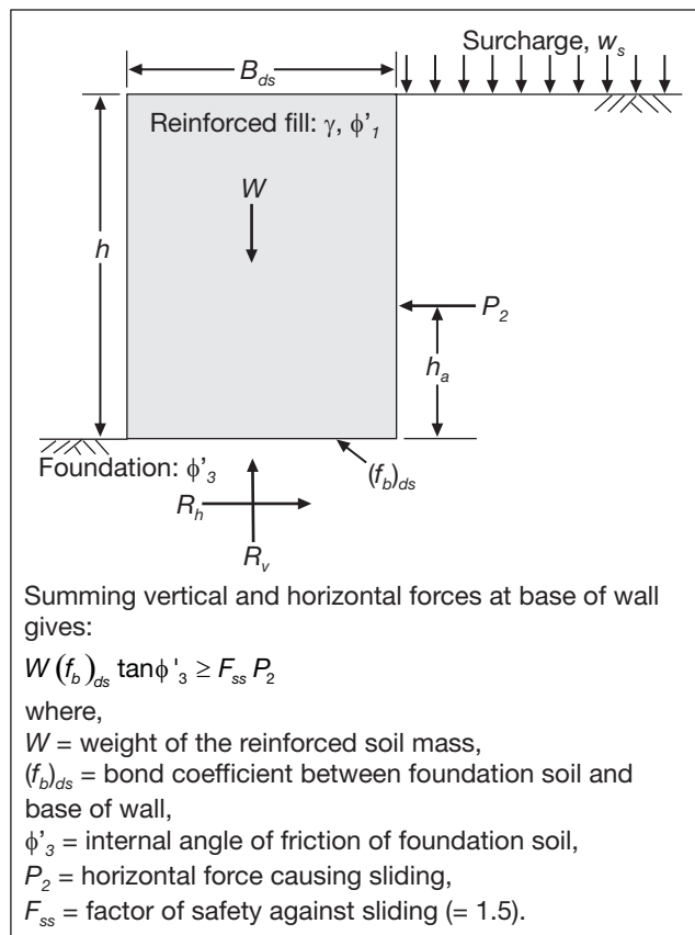
Figure 12 - Stability against sliding.
